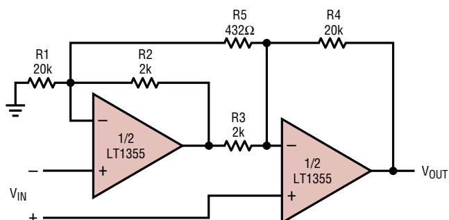
Instrumentation Amplifier
